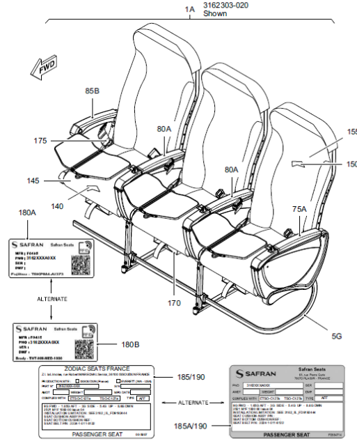
IAT Seat Assembly (Sheet 1 of 7) Figure 1A/Graphic-25-04-48-950-001-B01
